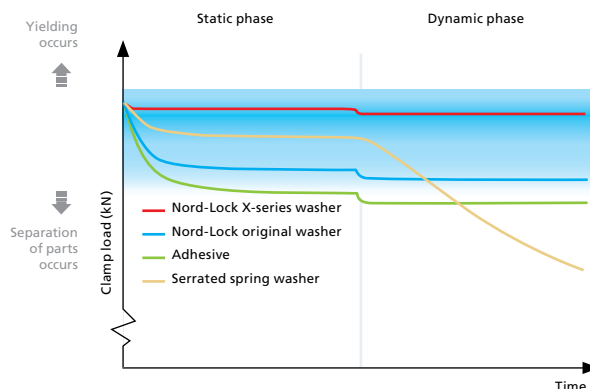
Fig 2: Tests show that Nord-Lock X-series performs better than any other alternatives currently available on the market when compensating slackening in static conditions and in preventing rotation of the fastener when the joint is exposed to vibration in the dynamic phase. With its unique, multifunctional solution, Nord-Lock X-series is the only product on the market that can secure bolts from both critical loosening factors at once. As shown in the graph, all bolted joints have a functional preload range in which the joint is safe. Serious problems start as soon as the preload falls outside the functional range. If the preload is too high, yielding occurs. If it is too low, there is separation or sliding between the parts. Only Nord-Lock X-series keeps you within the optimal limits.
